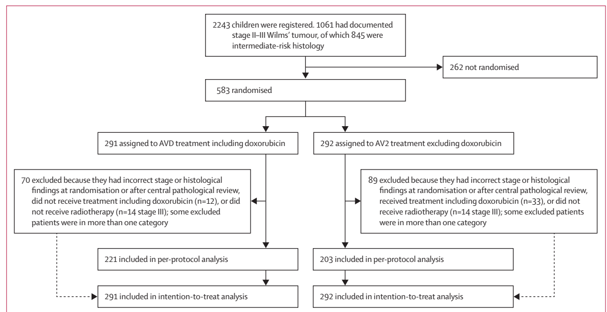
Figure 1: Trial profile
